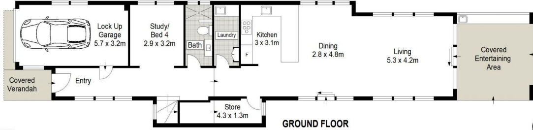
GROUND FLOOR
