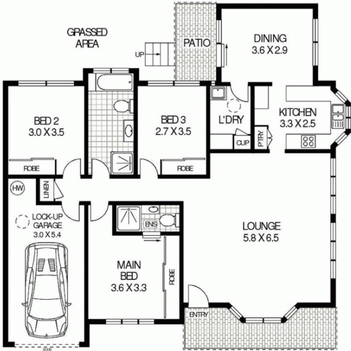
GROUND FLOOR
