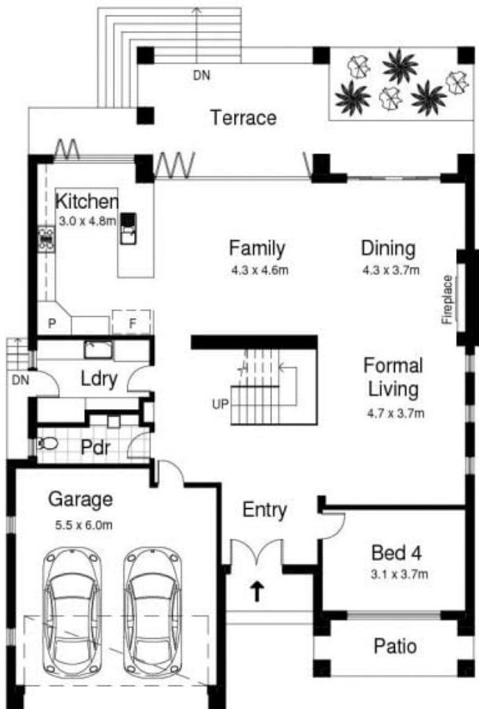
GROUND LEVEL
