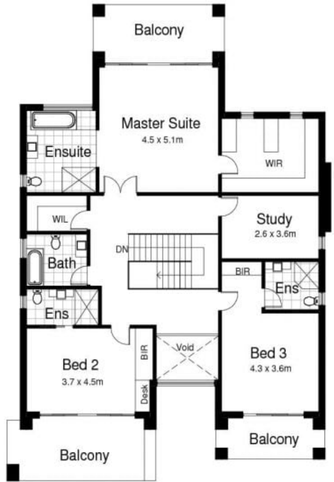
UPPER LEVEL
