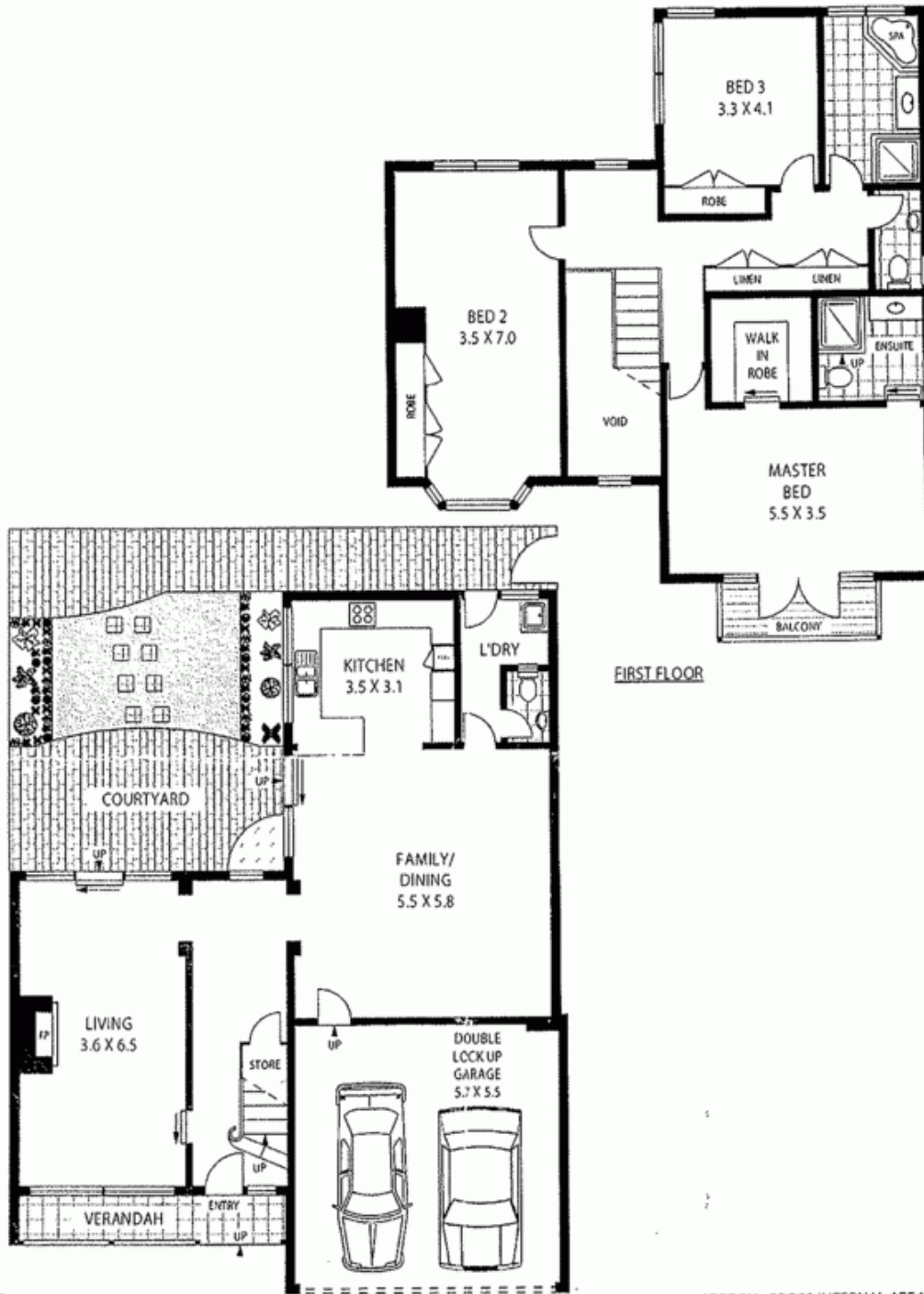
GROUND FLOOR
